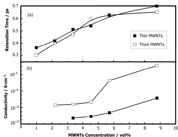
Fig.5 Relaxation time (a) and dc conductivity (b) vs. filler concentration for composites containing thin and thick MWNT.
