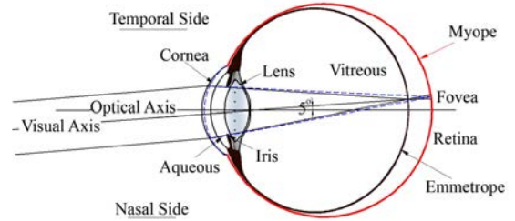
图 1 正视眼和近视眼的结构图以及角膜屈光手术的原理 Fig.1 Schematic diagram for emmetropic and myopic eye models, and the principle of refractive surgery.
