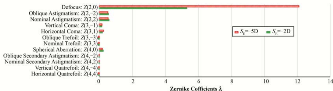
图3 -2D 和-5D 近视模型(6 mm)手术前波前像差系数 Fig.3 Wavefront aberration coefficients for -2D and -5D model (6 mm) before surgery.
