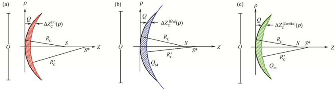
图 2 三种不同屈光手术的角膜“切削”量截面 (a) 球面修正, (b) Q 值优化, (c) 波前像差引导 Fig.2 Sectional view of ablation depth in three different refractive surgeries. (a) Spherical correction, (b) Q -value optimized, (c) Wavefront guided
