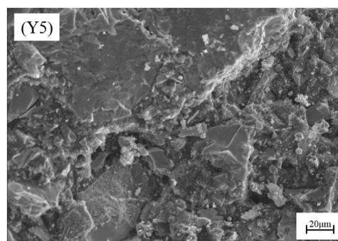
Fig. 10. SEM image of fracture surface of composite Y5 under irradiation.
