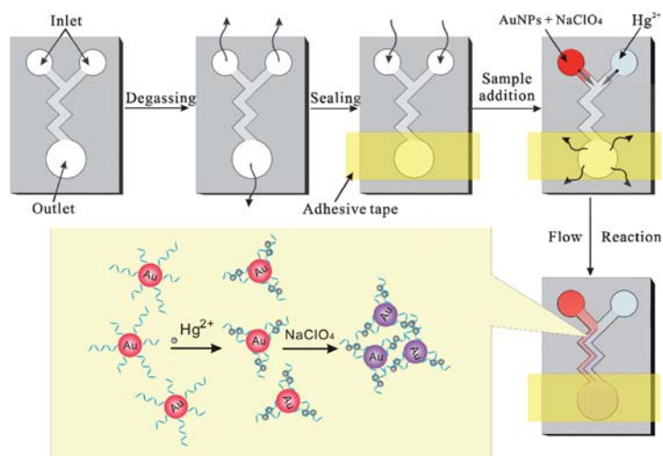
Fig. 1 Scheme for power-free \text{Hg}^{2+} sensing strategy. The black arrows in each step indicate the directions of air transfer. Also shown is the scheme for optical detection of \text{Hg}^{2+} using thymine-modified Au nanoparticles.
