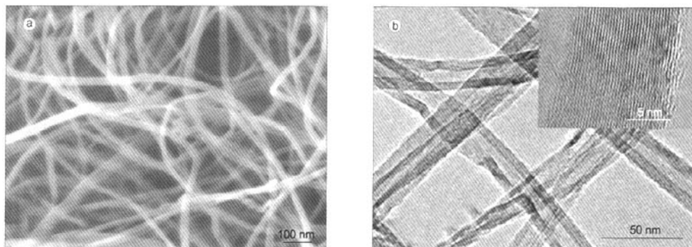
图1 初始碳纳米管的表面形貌和微观结构:(a)典型的SEM照片;(b)典型的TEM照片,内嵌为HRTEM照片 Fig. 1 Surface morphology and micro-structure of the as-grown CNTs: (a) typical SEM image, (b) typical TEM image and HRTEM image (the inset)
