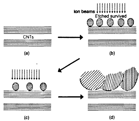
图5 石墨纳米晶形成及生长示意图. (a) 初始碳纳米管, (b) 甲烷和氢气混合离子沉积形成各种晶核取向的石墨晶核, (c) 晶面与离子束方向平行或成小角度的晶核保留, (d) 保留下来的晶核继续长大 Fig.5 The illustration of the formation and growth of nano-graphite. (a) initial CNTs, (b) disordered nano-graphite crystal nuclei induced by carbon hydrogen ions deposition, (c) the nano-graphite crystal nuclei survived with (002) planes parallel to the direction of ion beams or planes having small angles with the direction of ion beams, (d) the growth of retained crystal nuclei
