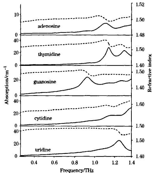
Fig. 2 THz absorption coefficient (solid line) and refractive index (dot line) of adenosine, thymidine, guanosine, cytidine and uridine
