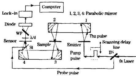
Fig. 1 Experimental setup for terahertz time-domain spectroscopy
