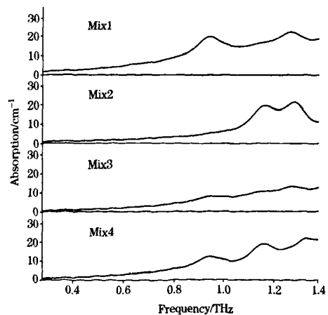
Fig. 3 THz absorption coefficient of the mixtures Mix1, Mix2, Mix3 and Mix4
